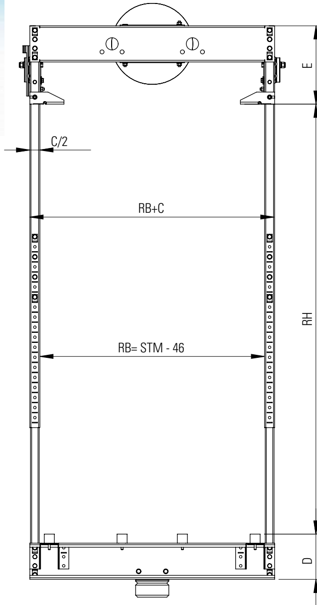
CF sm 1 pulley on top with SG, sliding guide shoes
